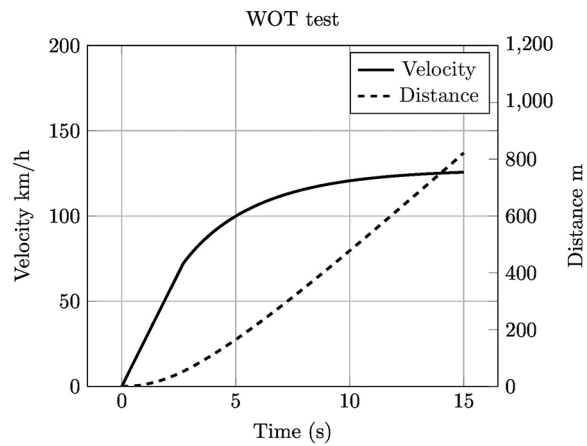
Fig. 4 WOT test of a fully loaded electric car and trailer
