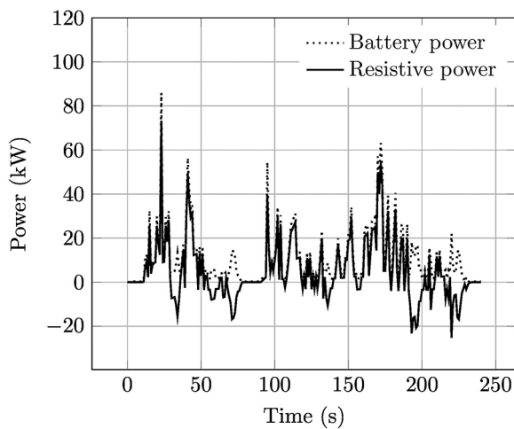
Fig. 5 Power flows during one SPC240 cycle
